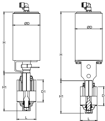
Pneumatic Weld Butterfly Valve 不锈钢气动焊接蝶阀
