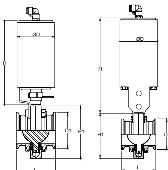
Pneumatic Clamp Butterfly Valve 不锈钢气动快装蝶阀
