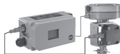
Fig. 4: Type 3730-5 External position sensor with Type 3510 Micro-flow Valve
